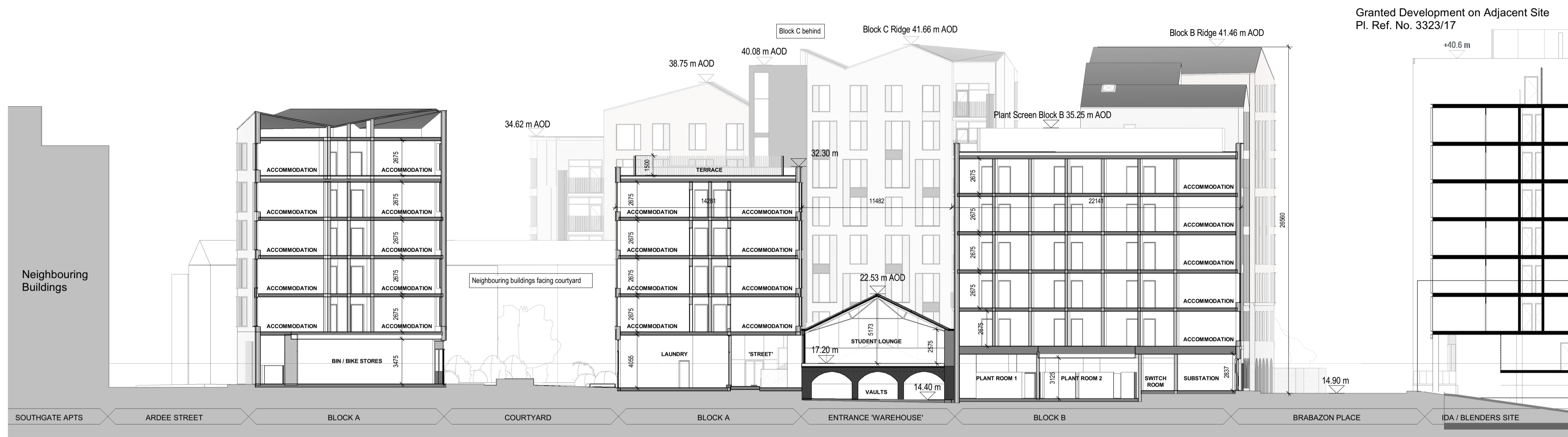
1 Section AA - through Block A courtyard facing North 1 : 200
