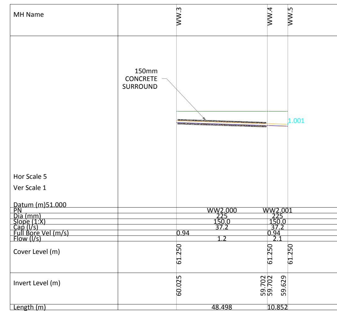
WASTEWATER NETWORK (WW2.000)
