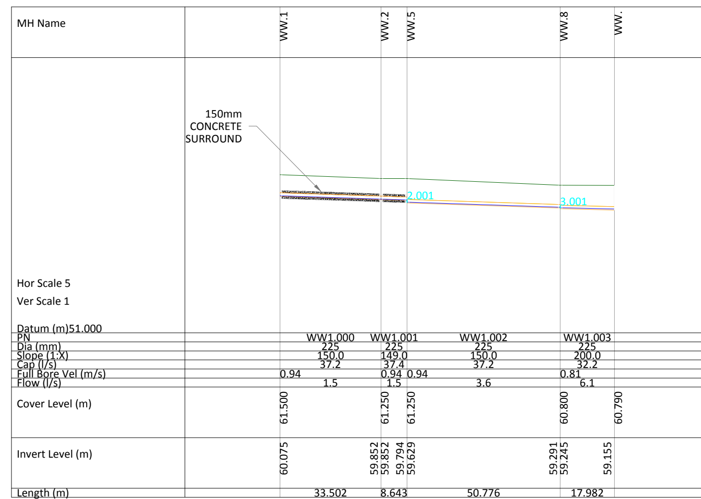
WASTEWATER NETWORK (WW1.000)
