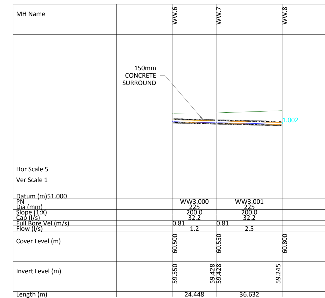
WASTEWATER NETWORK (WW3.000)
