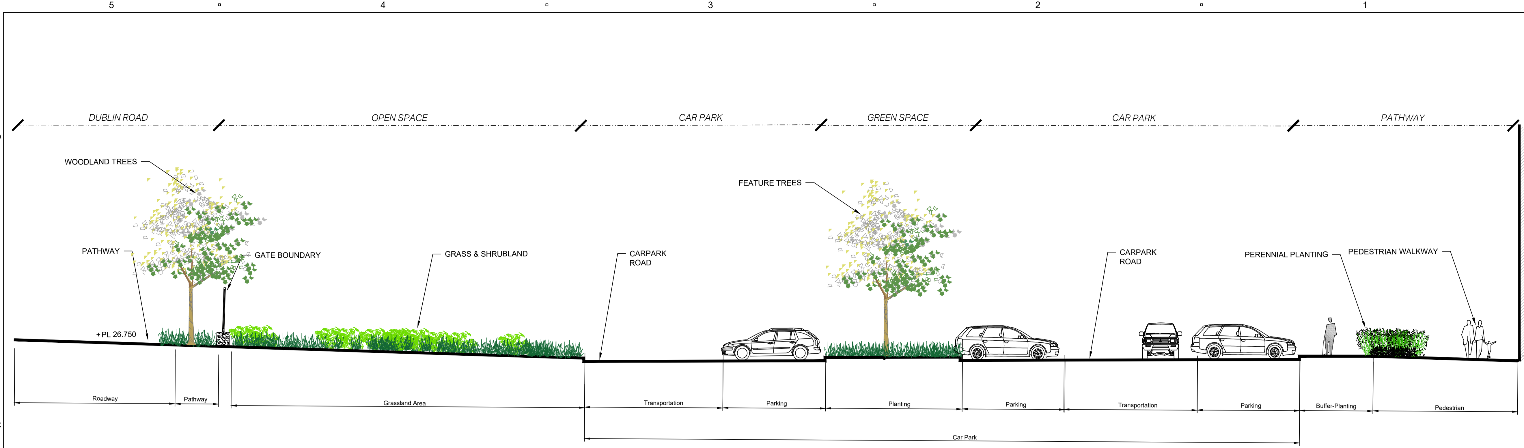
8 CAR PARK INTERFACE BLOCK G (H-H) SCALE: 1:100
