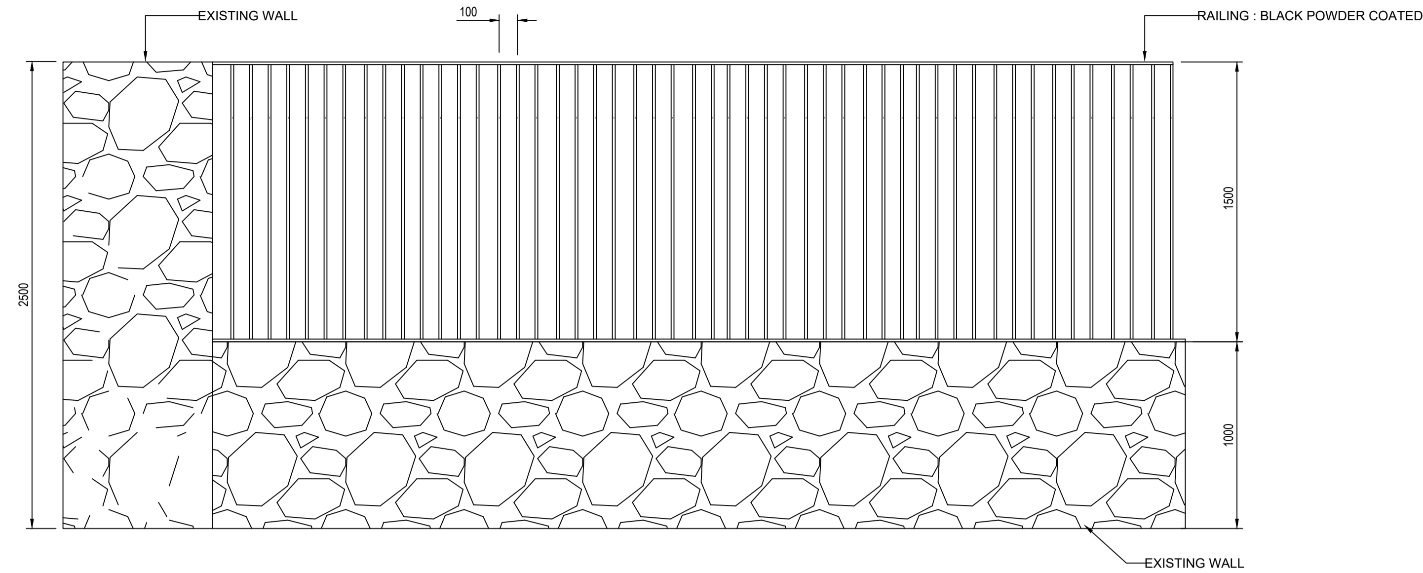
09 STEEL RAILING ON LOWERED SECTION OF THE EXISTING STONE WALL 7004 SCALE: 1:20 @A1
