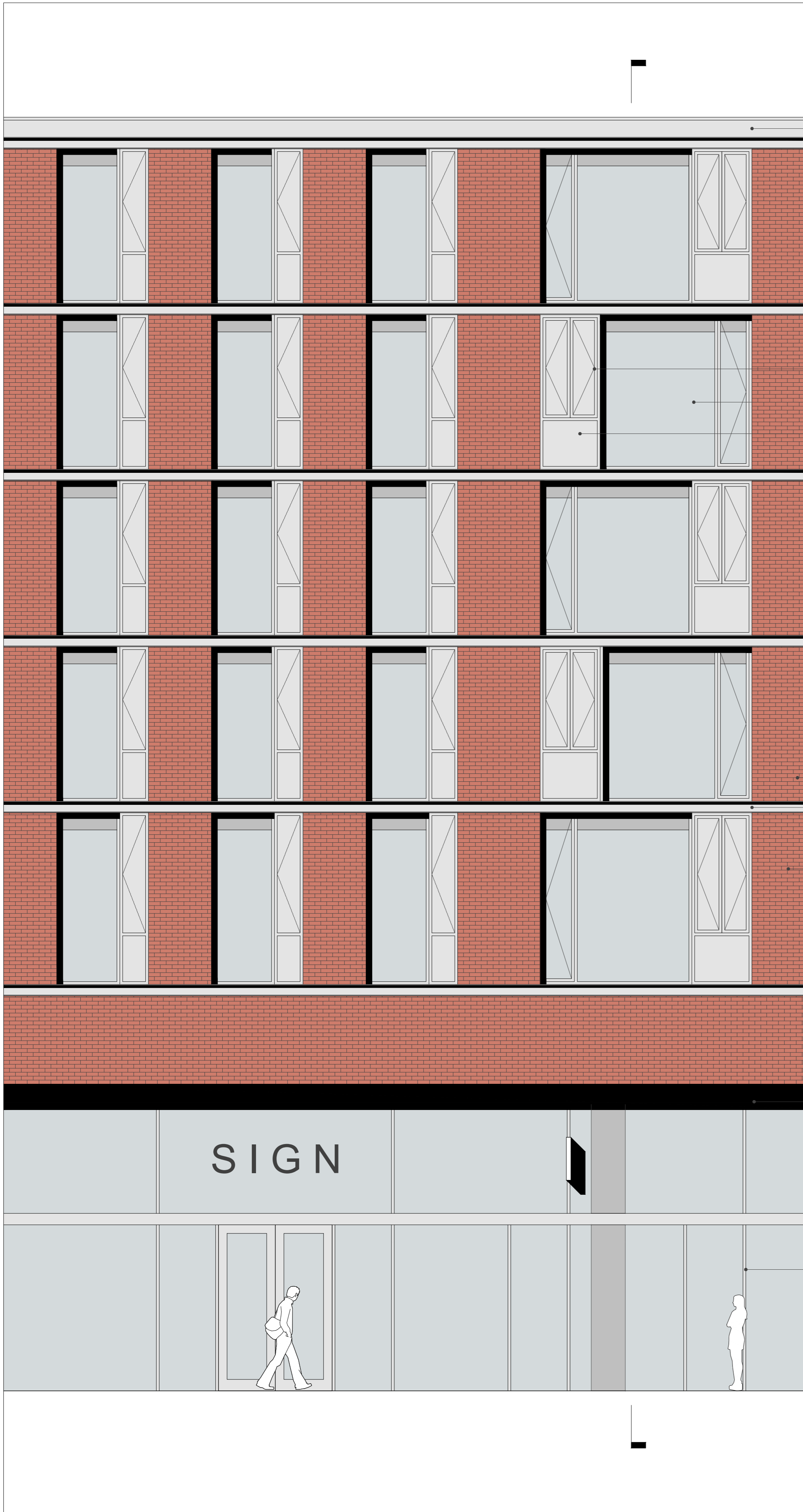
ELEVATION: 1:50
