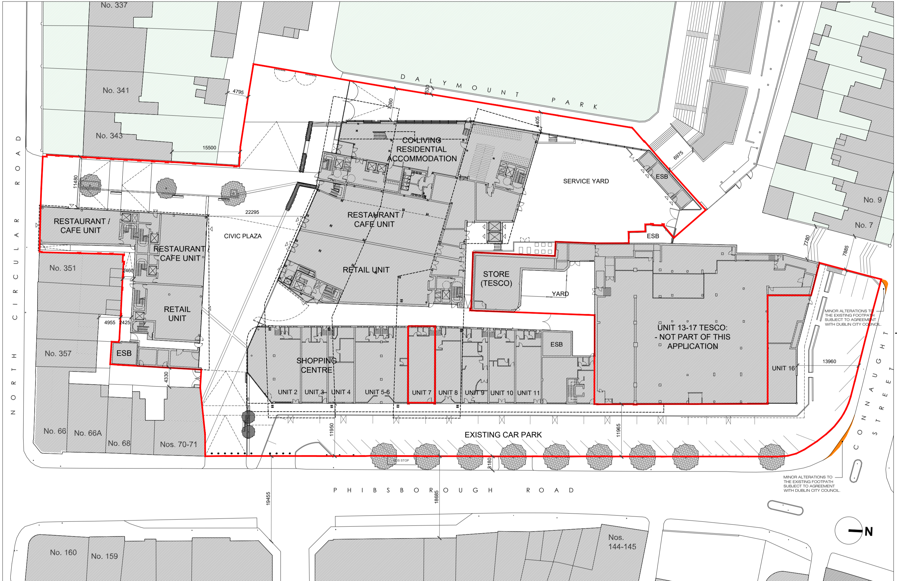
PROPOSED SITE LAYOUT PLAN 1:500@A1
