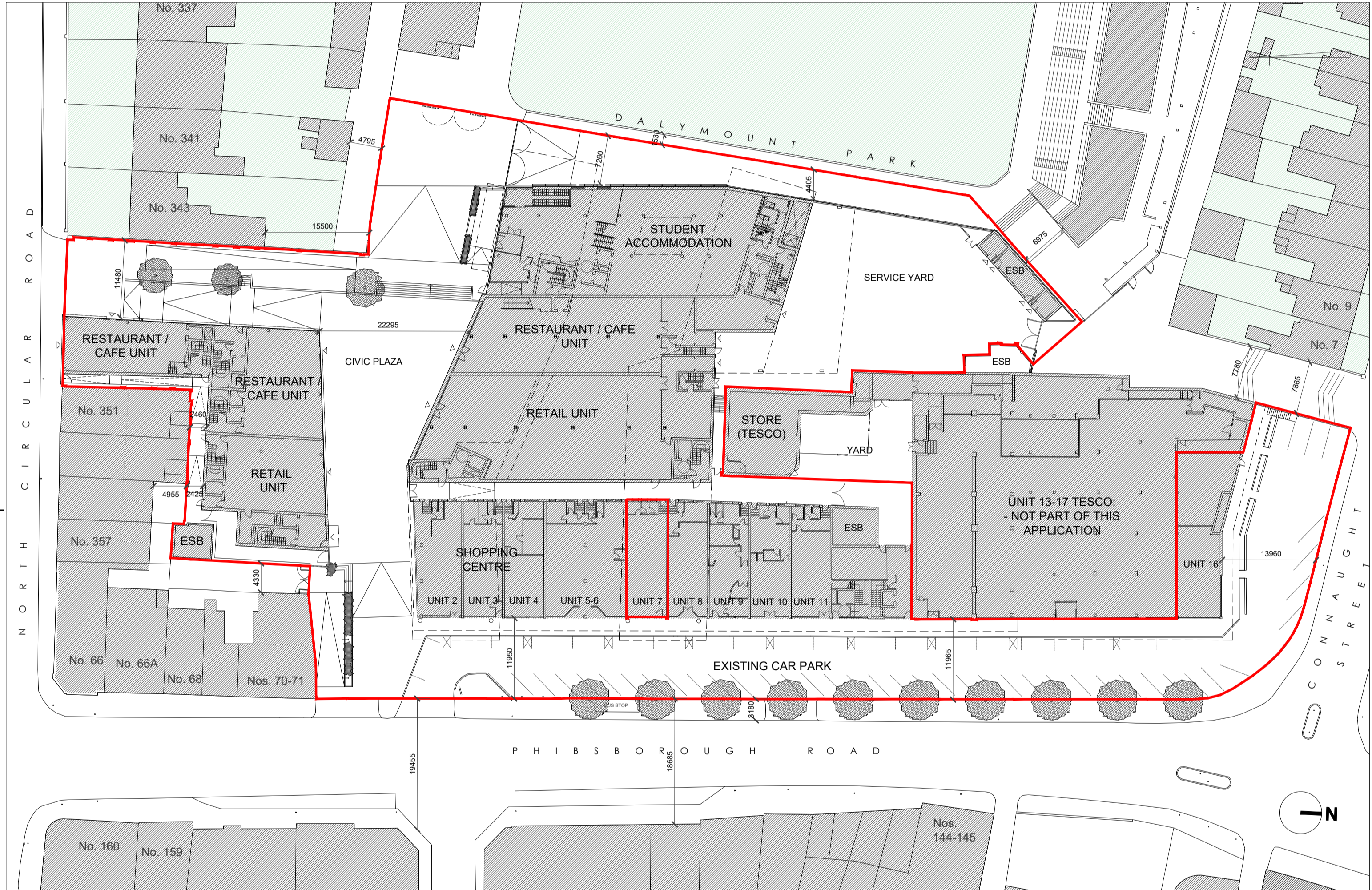
PERMITTED SITE LAYOUT PLAN 1:500@A1 (A.B.P. ref. 300241-17 AUGUST 2018)
