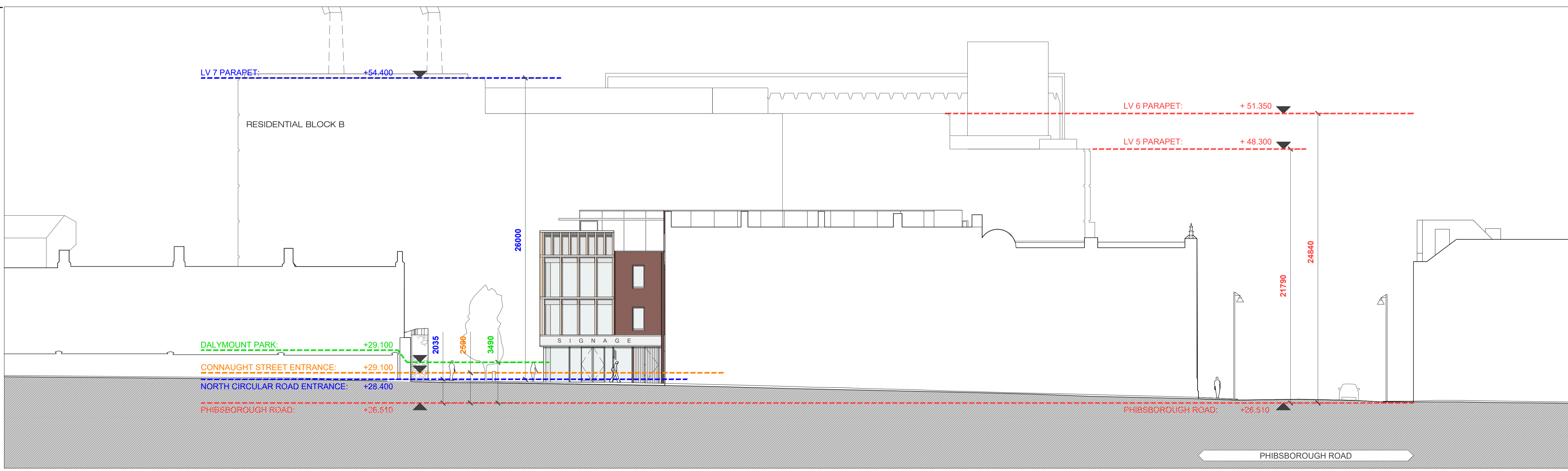
PROPOSED ELEVATION: NORTH CIRCULAR ROAD
